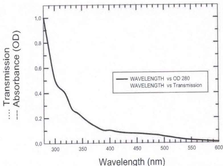
Figure 6. Absorption and Transmission of AC-11 as thin film* in deionized water. [AC-11] = 40 mg/ml *Three drops of above solution were dried overnight onto a methacrylate disposable UV grade 1.0 cm cuvette (Sigma Chemical Co.).
